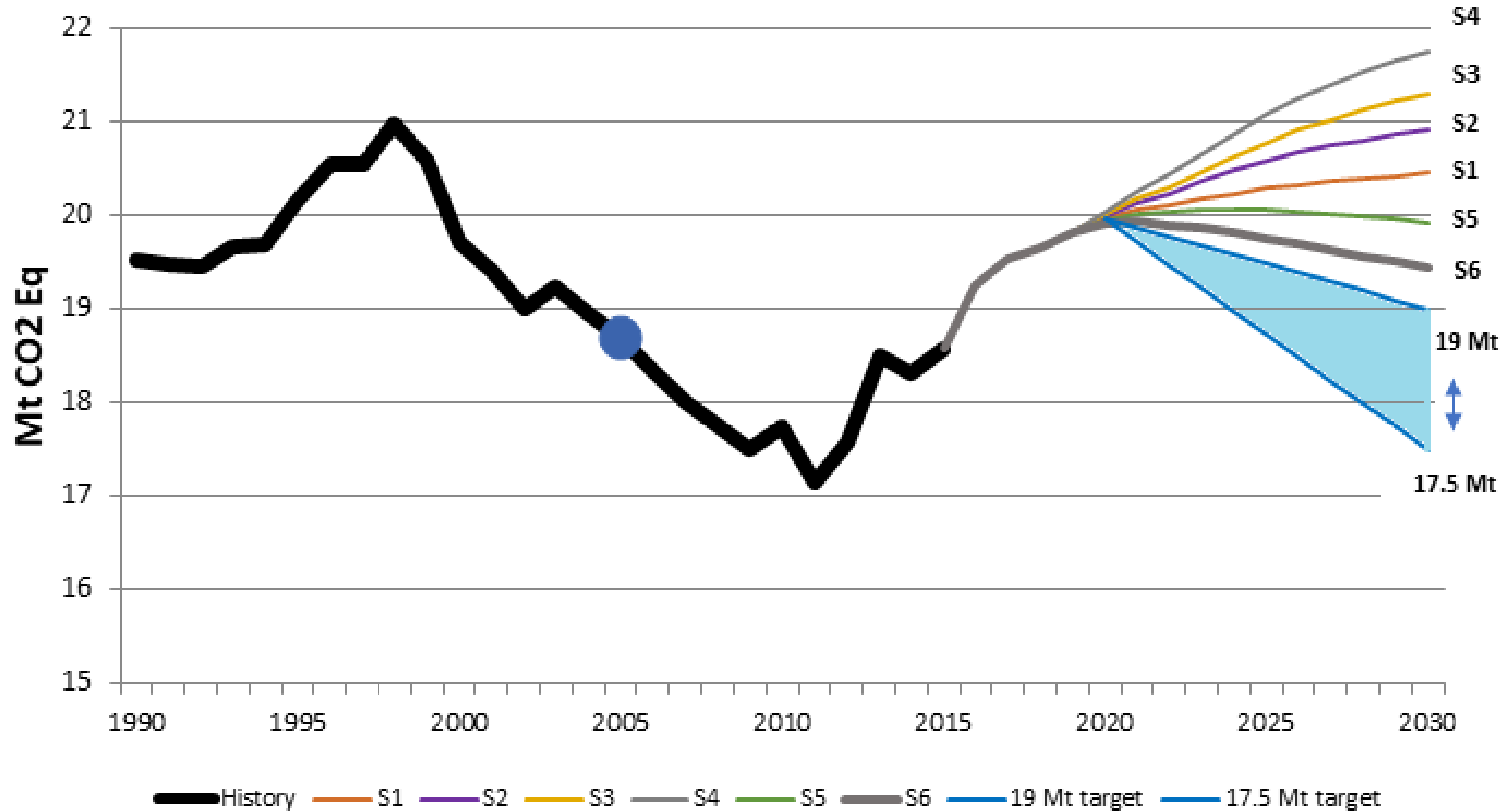
Teagasc Scenarios 1-6 against the required emissions target range (blue) for 2030 (excludes mitigation measures)
